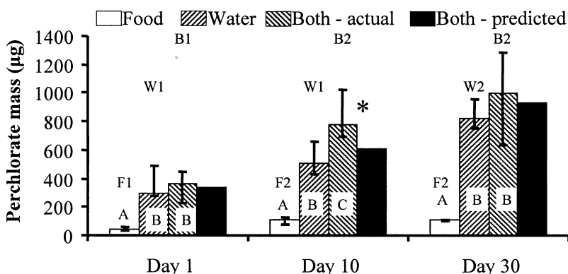
Figure 3. Perchlorate total mass (µg) in largemouth bass exposed to perchlorate via food only, water only or both food and water for 1- 30 days. Bars represent medians and error bars are first and third quartiles. Bars labeled with different letters are significantly different for comparisons among treatments within exposure durations only ( p > 0.05 , Kruskal-Wallis test). Alphanumeric labels (e.g., F1, W2, etc.) denote significant differences between exposure durations within each treatment: Food only (F), water only (W), and both food and water (B). Asterisks denote significant differences between observed and predicted values for body burdens in the “both water and food”.
